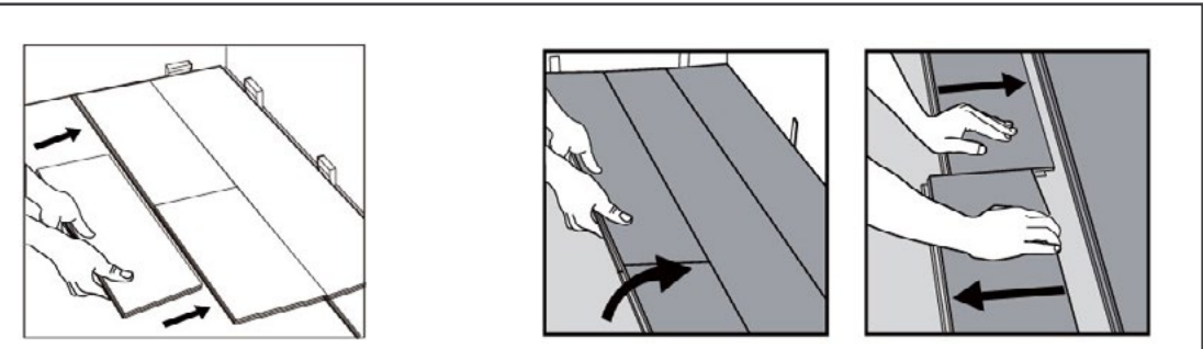
Step 7 Pull bar and rubber mallet can be used for final row of planks, ensuring an expansion gap is Minimum of 3/8" or thickness of the plank whatever is greater.
