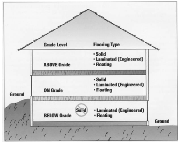
If any part of the soil surrounding a structure is above the floor of any level, consider that level below-grade. This includes walk-out basements. In addition, the surrounding soil should be sloped away from the structure with at least 6 inches of fall over the first 10 feet.
