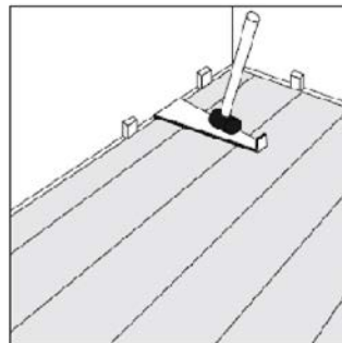
Step 7 Pull bar and rubber mallet can be used for final row of planks, ensuring a 1/2" expansion gap
