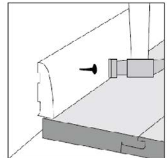
Step 8 Refitting of skirting board with hidden 1/2" expansion gap
