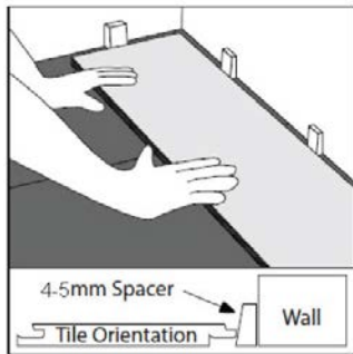
Step 1 Laying first plank in corner of room with tongue side facing wall using 1/2" spaces
