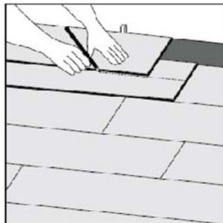
Step 6 Measure and cut final row of planks allowing for 1/2" expansion gap
